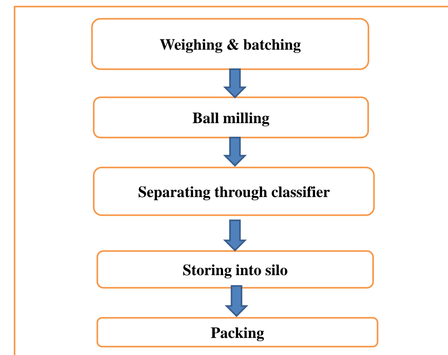
Fig.3 Schematics of grinding process
